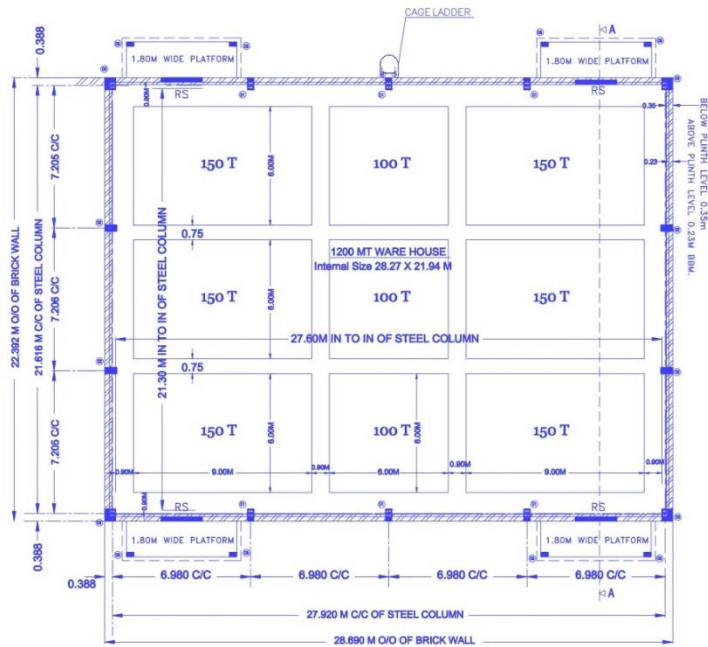
PLAN FOR 1200 MT WARE HOUSE UNIT
